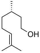
(S)-Citronellol 38%
