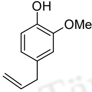
Eugenol
