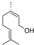
Nerol 7%
